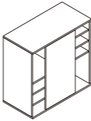
Model TG03-B Size 800(W)*400(D)*1960(H)mm
